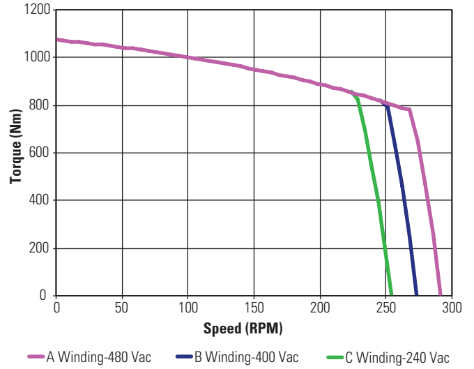
KBM(S)-163X02 Continuous Torque
