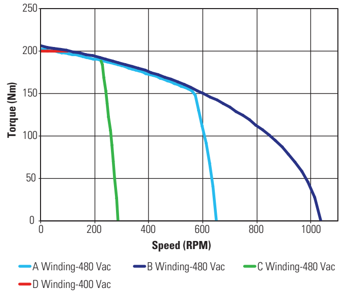
KBM(S)-88X01 ContinuousTorque
