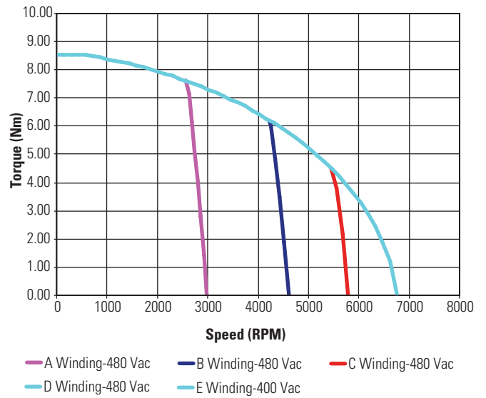
KBM(S)-25X02 ContinuousTorque
