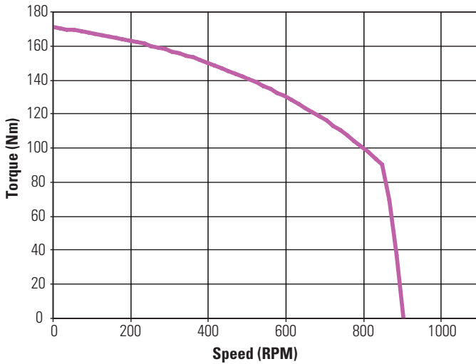
KBM(S)-118X00 ContinuousTorque
