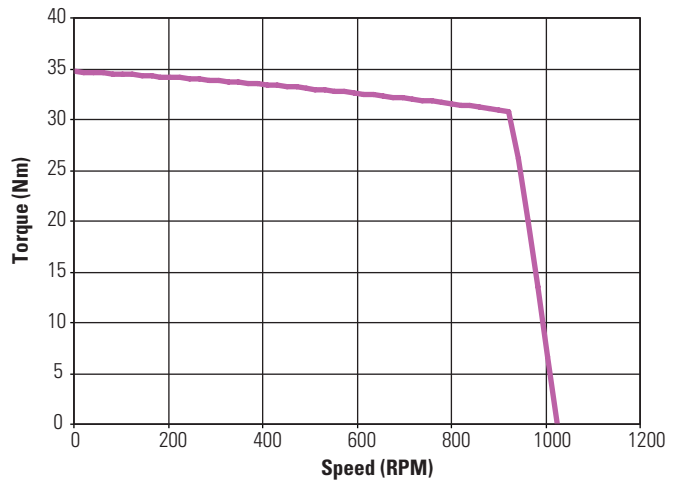
KBM(S)-43X04 ContinuousTorque
