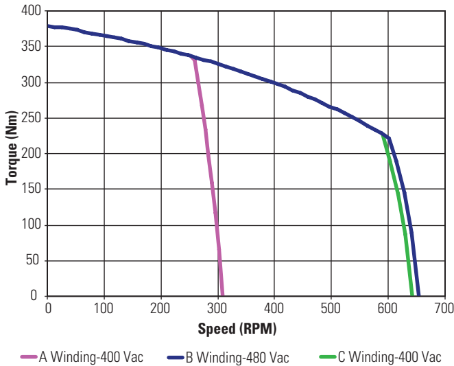
KBM(S)-88X02 ContinuousTorque
