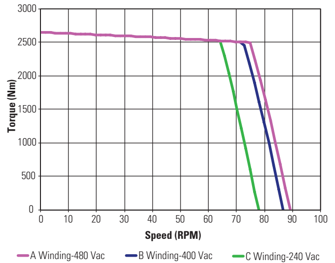
KBM(S)-260X02 Continuous Torque
