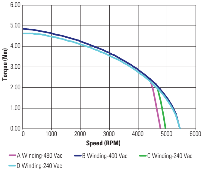
KBM(S)-25X01 ContinuousTorque
