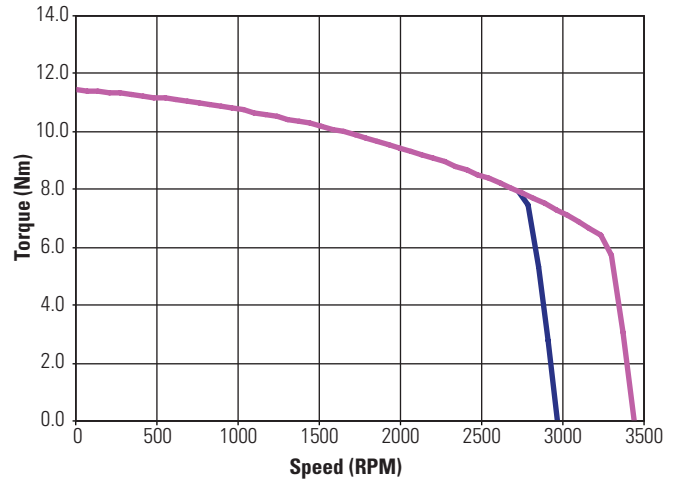
KBM(S)-43X02 ContinuousTorque
