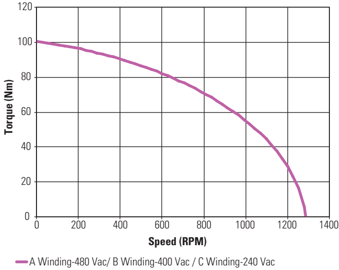
KBM(S)-88X00 ContinuousTorque
