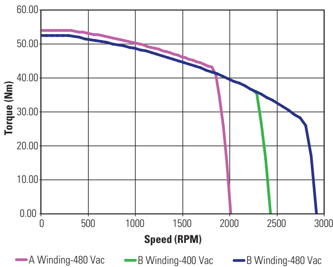
KBM(S)-45X03 Continuous Torque
