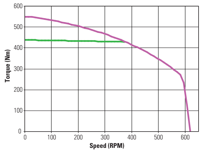
KBM(S)-118X03 ContinuousTorque
