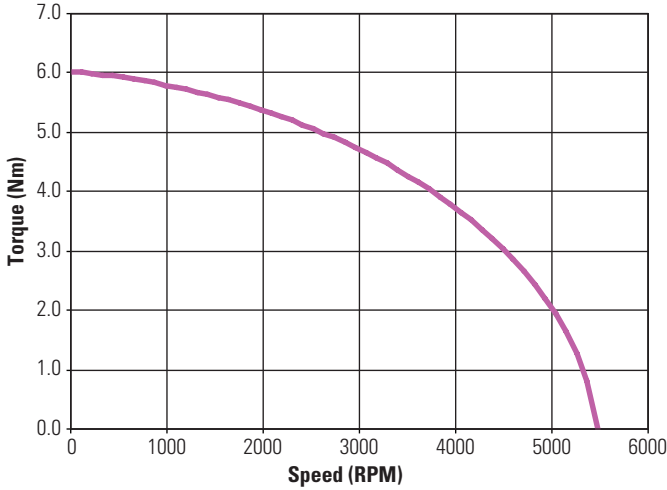
KBM(S)-43X01 ContinuousTorque
