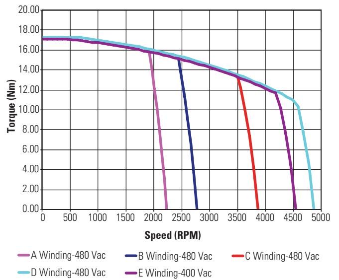
KBM(S)-35X02 Continuous Torque
