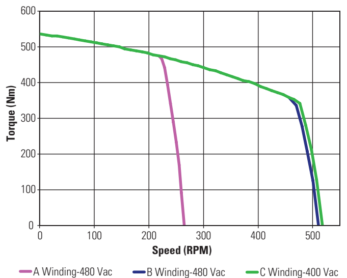
KBM(S)-88X03 ContinuousTorque
