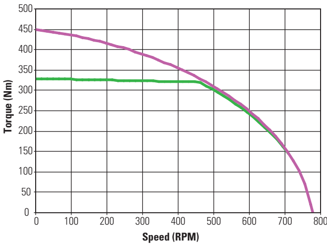
KBM(S)-118X02 ContinuousTorque
