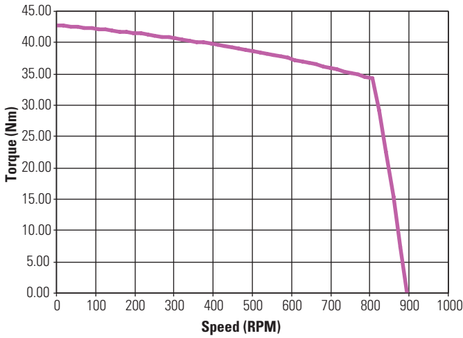
KBM(S)-79X01 ContinuousTorque
