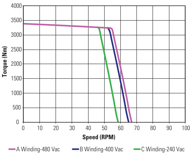
KBM(S)-260X03 Continuous Torque
