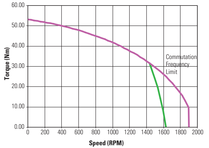
KBM(S)-60X01 Continuous Torque
