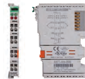
I/O bus terminal modules Front connections and side view
