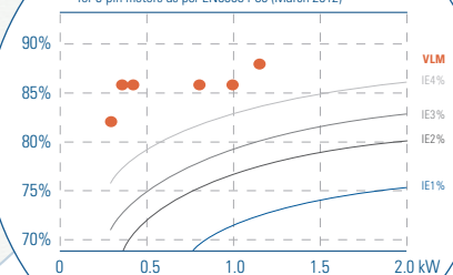
VLM efficiency and IE classification for 6-pin motors as per EN60034-30 (March 2012)
