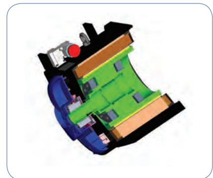
Design of a Cartridge DDR motor (CDDR)
