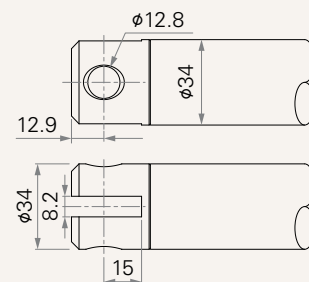
4 = #45 Steel, U clevis, slot 8.2, depth 15.0, hole 12.8
