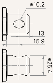
5 = Stainless Steel, slotless, hole 10.2
