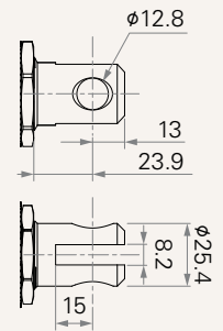
8 = Stainless Steel, U clevis, slot 8.2, depth 15.0, hole 12.8
