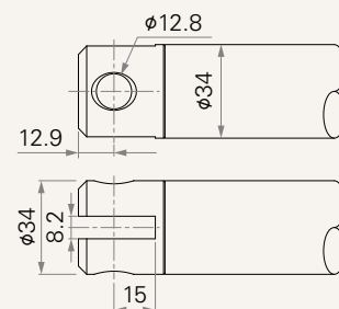
8 = Stainless Steel, U clevis, slot 8.2, depth 15.0, hole 12.8
