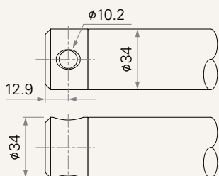
5 = Stainless Steel, slotless, hole 10.2
