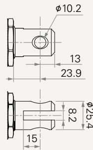
7 = Stainless Steel, U clevis, slot 8.2, depth 15.0, hole 10.2
