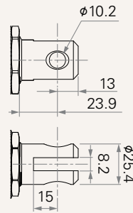
3 = #45 Steel, U clevis, slot 8.2, depth 15.0, hole 10.2
