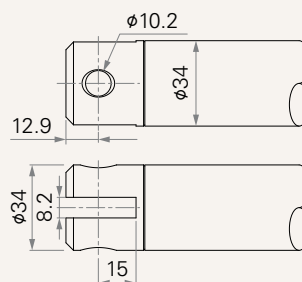
7 = Stainless Steel, U clevis, slot 8.2, depth 15.0, hole 10.2
