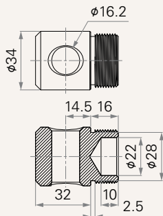
9 = #45 Steel, slotless, hole 16.2
