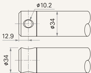
1 = #45 Steel, slotless, hole 10.2
