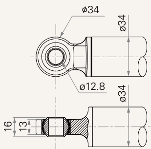
K = Rod end bearing, hole 12.8
