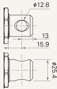
6 = Stainless Steel, slotless, hole 12.8
