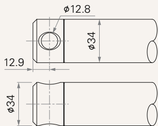
2 = #45 Steel, slotless, hole 12.8
