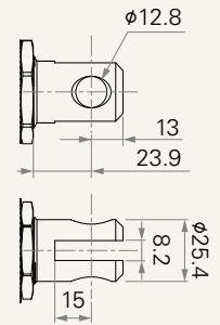
4 = #45 Steel, U clevis, slot 8.2, depth 15.0, hole 12.8
