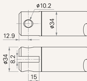
3 = #45 Steel, U clevis, slot 8.2, depth 15.0, hole 10.2
