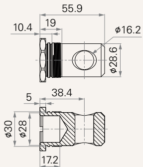
9 = #45 Steel, slotless, hole 16.2
