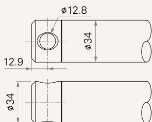
6 = Stainless Steel, slotless, hole 12.8
